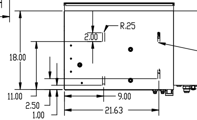
MOUNTING SLOTS .5 X 2.00 FOUR PLACES
